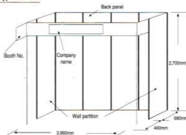
Type S booth
