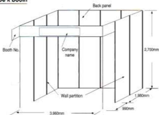
Type R booth
